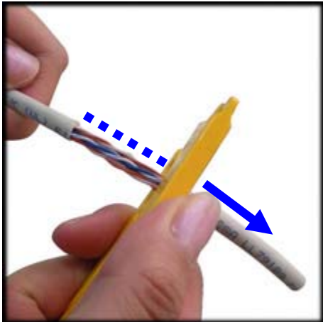
STEP 3 Stripper UTP/STP Jacket
