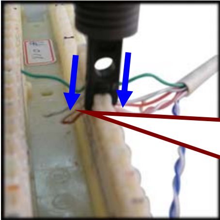
Punch down and cut wire (RP-PD224C)
